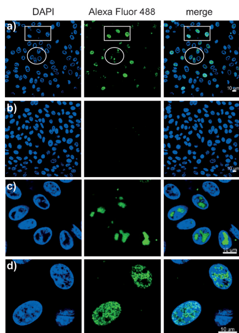
Figure 3. a) Vero cells infected with HSV-1 (multiplicity of infection (MOI) = 10) were incubated with dF-EdU (10 \mu M) for 8 h, fixed, and stained with azide-conjugated Alexa Fluor 488 in the presence of Cu I . b) Control samples were treated identically but received no HSV-1. c) High-magnification images illustrating labeling of the viral replication compartments. d) High-magnification images illustrating labeling of cellular nucleic acids. Scale bars: 10 \mu m.
