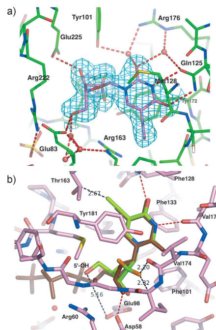
Figure 2. a) Cocrystal structure of dF-EdU (violet) bound in the active site of HSV1-TK (green, PDB entry code 4OQL). The electron density map ( 2F_{\text{obs}} - F_{\text{calc}} ) of dF-EdU with a resolution of 2.1 Å is contoured at 1 \sigma and shown in cyan. Water molecules are depicted as red spheres and hydrogen bonds as dashed red lines. b) Superposition of dF-EdU (green) onto dTTP (brown) within the active site of hTK (pink, PDB entry code 1W4R). [22]
